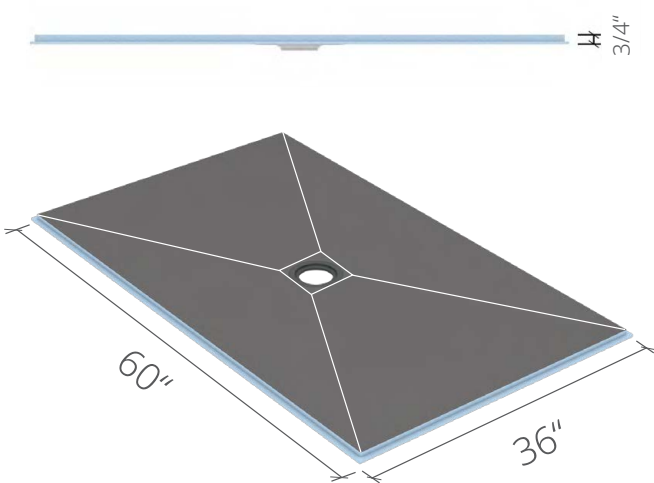
wedi Fundo® Curbless Shower Base 36 in. × 60 in. × 3/4 in. US9200003
