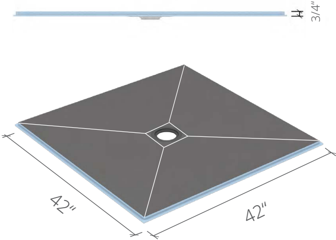
wedi Fundo® Curbless Shower Base 42 in. × 42 in. × 3/4 in. US9200006
