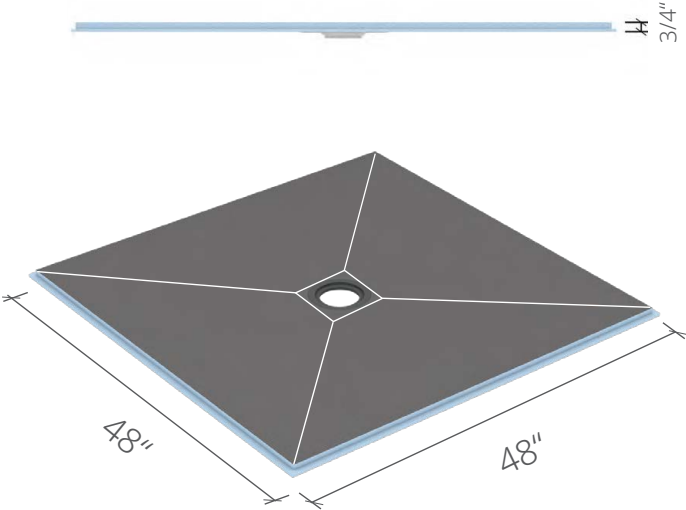
wedi Fundo® Curbless Shower Base 48 in. × 48 in. × 3/4 in. US9200002
