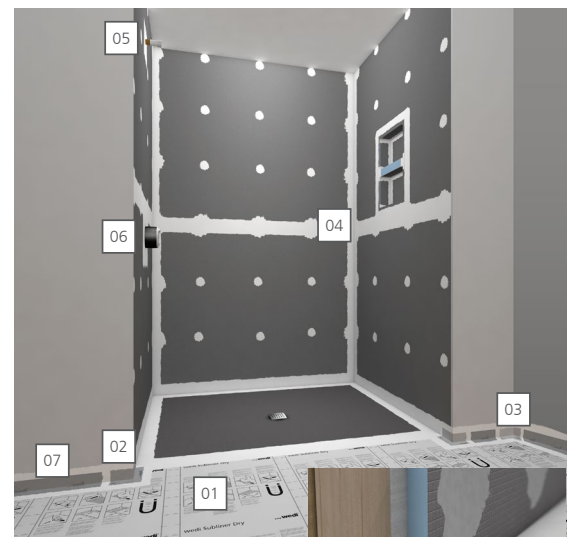
wedi Fundo Ligno Shower installation with Subliner Dry System
